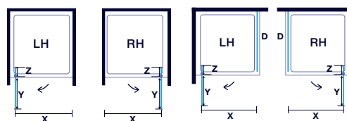
Pivot Door in Recess
