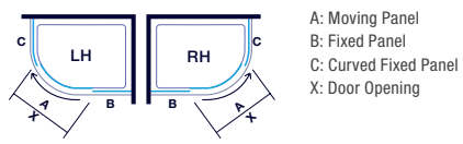
1 Door Offset Quadrant
