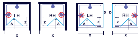
Bifold Door in Recess
