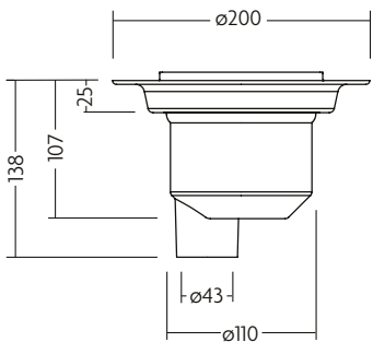
Vertical Outlet
