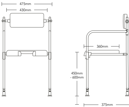
Freestanding Shower Chair Code: S5/
