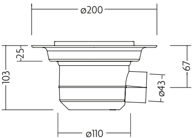
Horizontal Outlet
