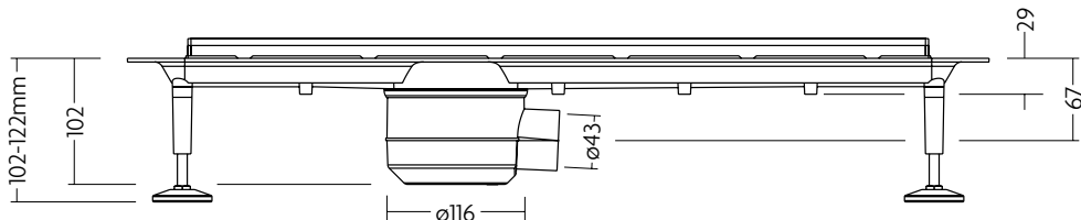
Horizontal Outlet
