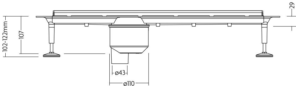
Vertical Outlet
