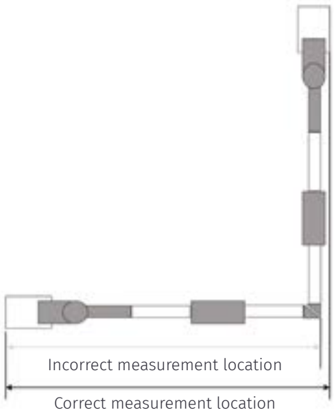
Correct measurement location
