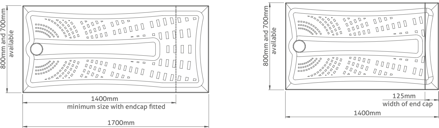
When measuring and cutting the tray please allow for the the end cap.
